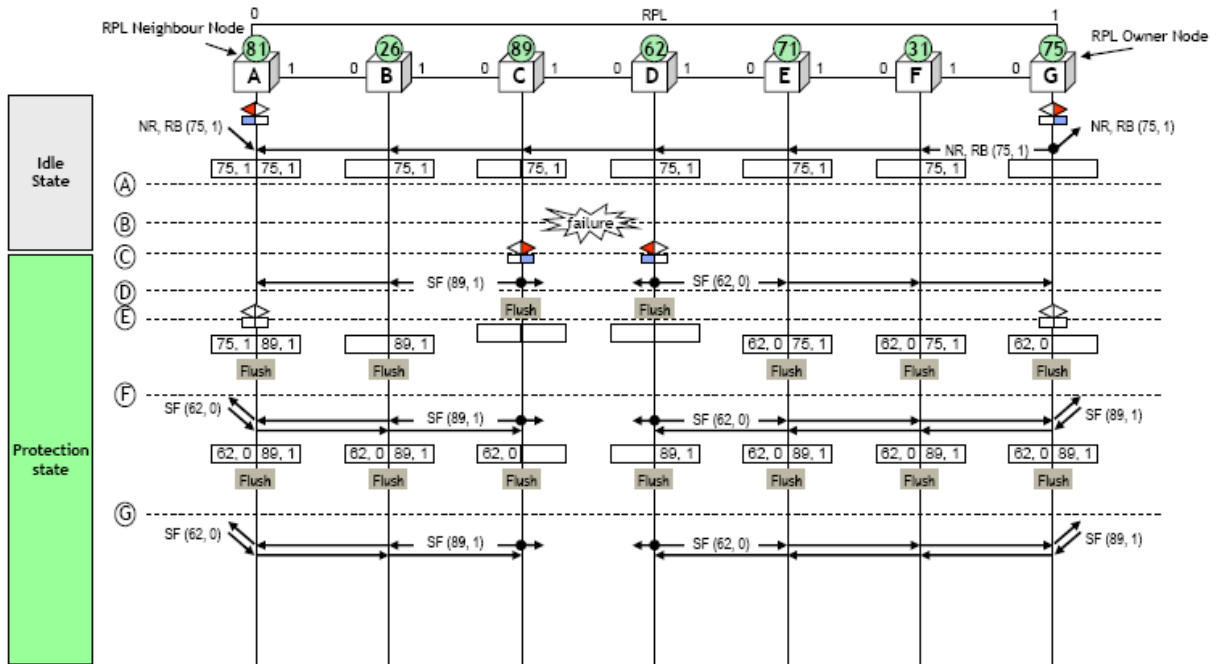
Figure 7-14 single-link fault
