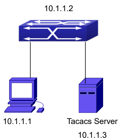
Figure 6-20 TACACS Configuration
