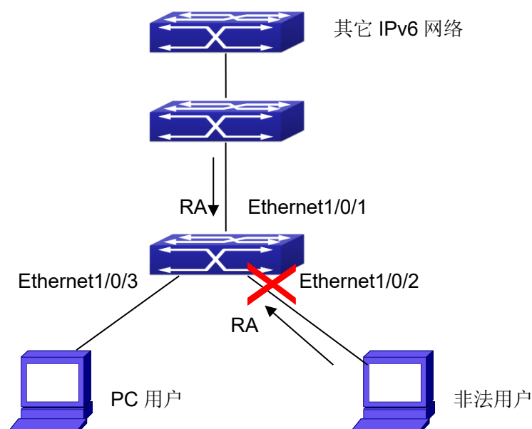
Figure 12-8 IPv6 Security RA sketch map
