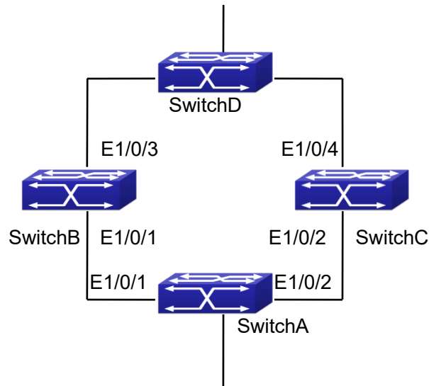
Figure 7-13 ULSM typical example
